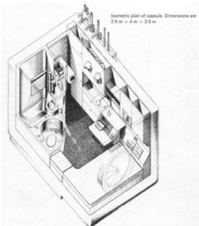
Fig 3. Nakagin Capsule Tower de Kisho Kurokawa, 1972.
