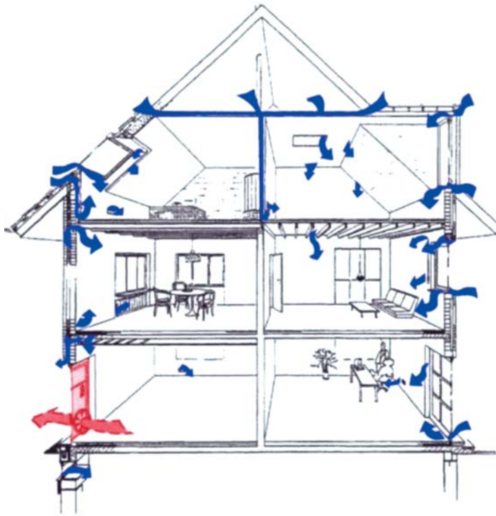
Figura 3. Test BlowerDoor.
